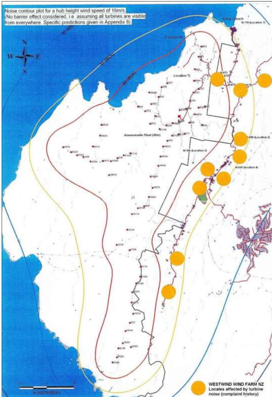
Approximate noise contours generated by the developer on the basis of Vestas V90 turbines
