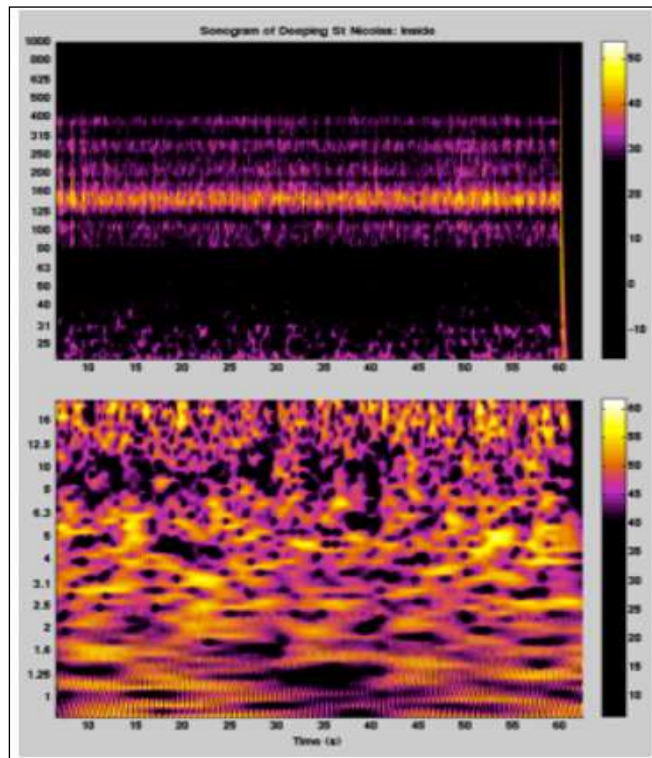
Figure 9: sound of wind turbines at 930 metres, inside residence
