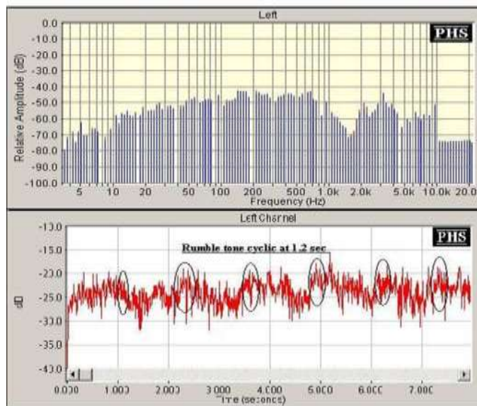
Figure 14: Turbine rumble
