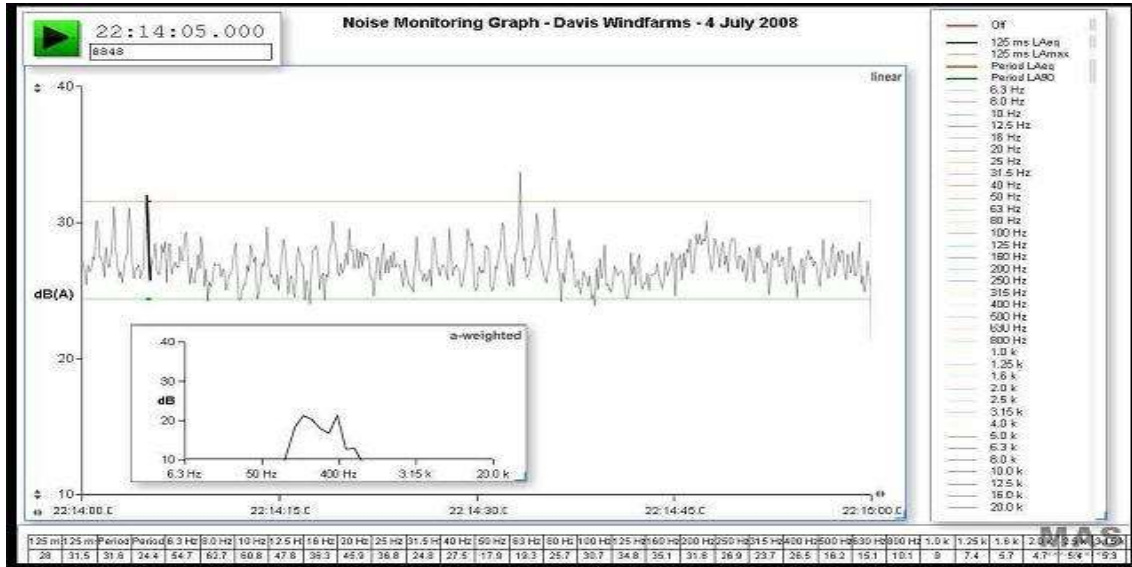
Figure 8: sound of wind turbines at 930 metres, inside residence
